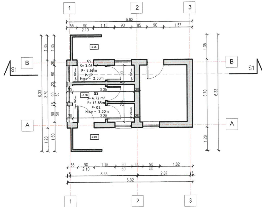
Wc public Daia - Plan parter Public WC Daia - Ground floor
