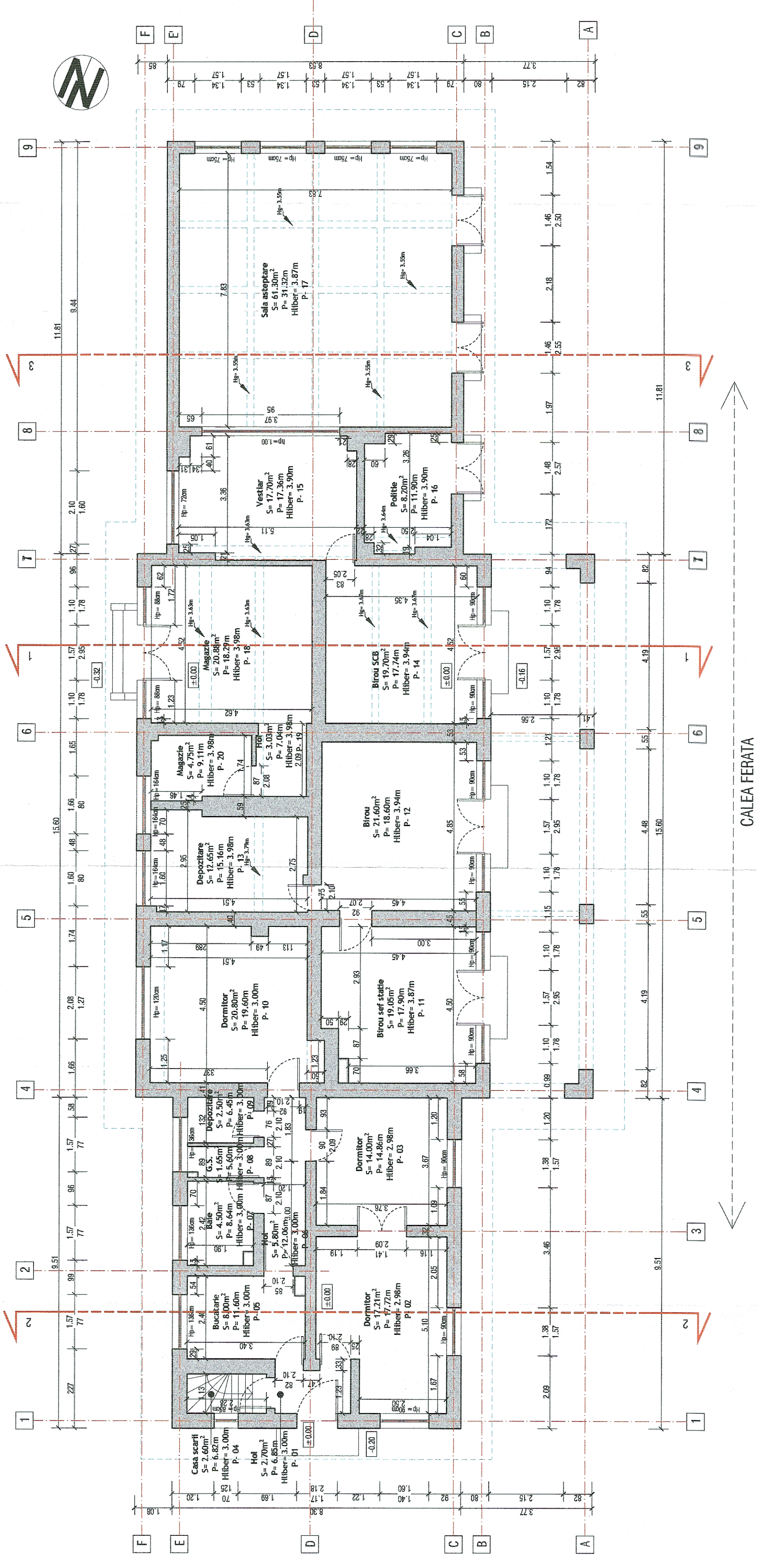
Clădire de călători Jilava - Plan parter / Train station building Jilava - Ground floor
