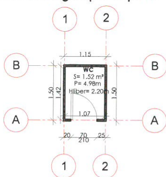
WC public Halta Aghireș - Plan parter
