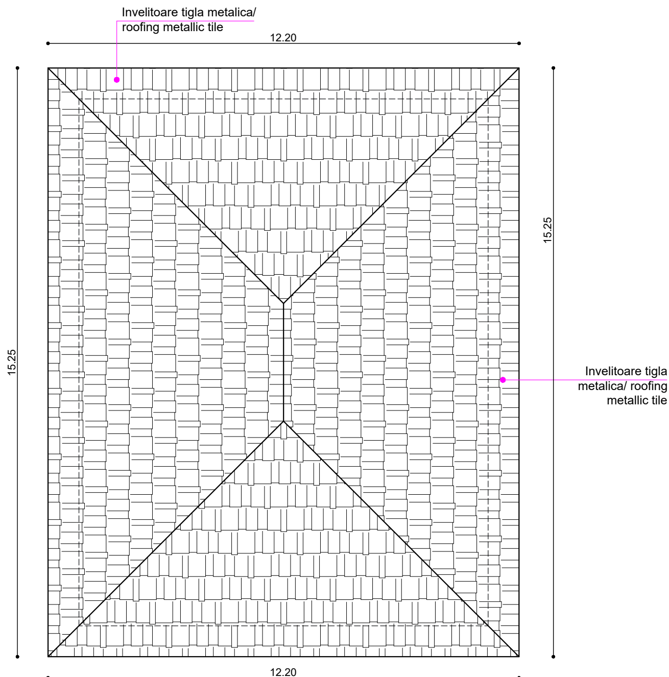
PLAN INVELITOARE/ ROOFTOP PLAN
