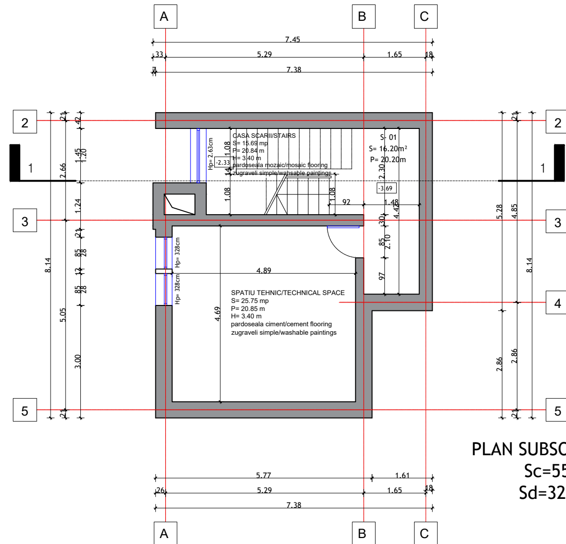
Plan subsol/ Basement
