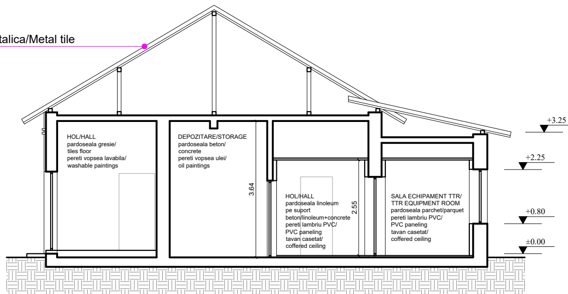
Cladire Politie (fosta CED)/Police Building (former CED) Sectiune A - A/Section A - A sc 1:100
