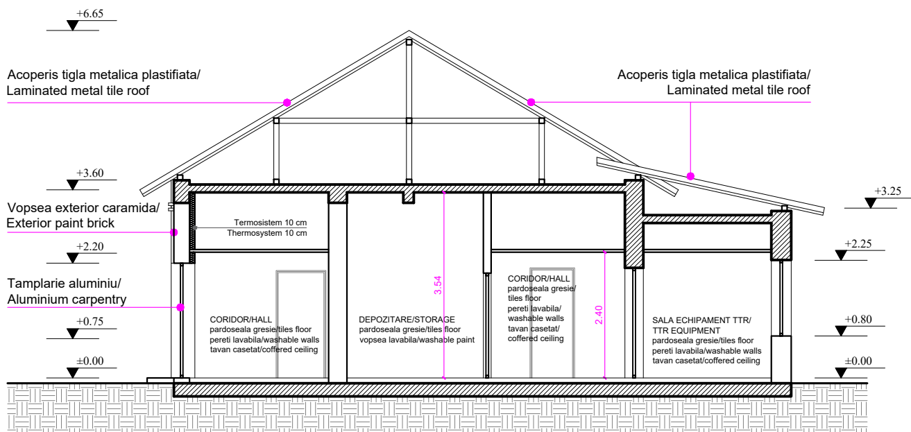
Cladire Politie/Police Building Sectiune A - A/Section A - A sc 1:100
