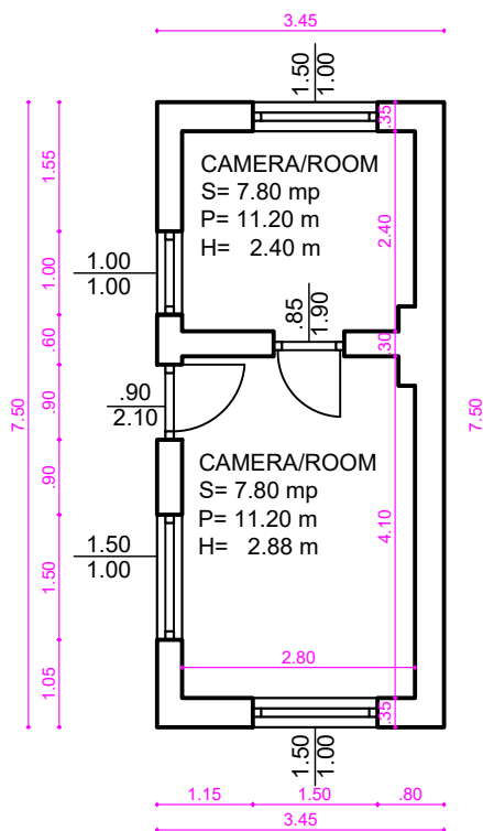
Clădire post mișcare 5/ Post movement building 5 Plan parter/ Ground floor plan sc 1:100 A_{construita} = 25.60 \text{ mp} A_{desfasurata} = 25.60 \text{ mp} P = 21.90 \text{ m}
