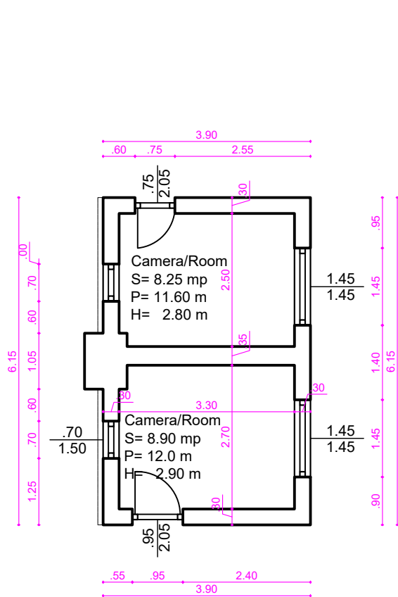
Cabină acari 8/ Pointsman's Cabin 8 Plan parter/ Ground Floor sc 1:100 A construita = 24.00 mp A desfasurata = 24.00 mp P = 20.10 m
