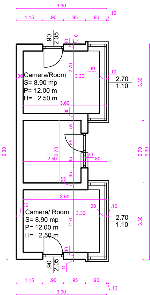
Cabină acari post 6/ Pointsman's Cabin 6 Plan parter/ Ground Floor sc 1:100 A construita = 34.10 mp A desfasurata = 34.10 mp P = 28.00 m
