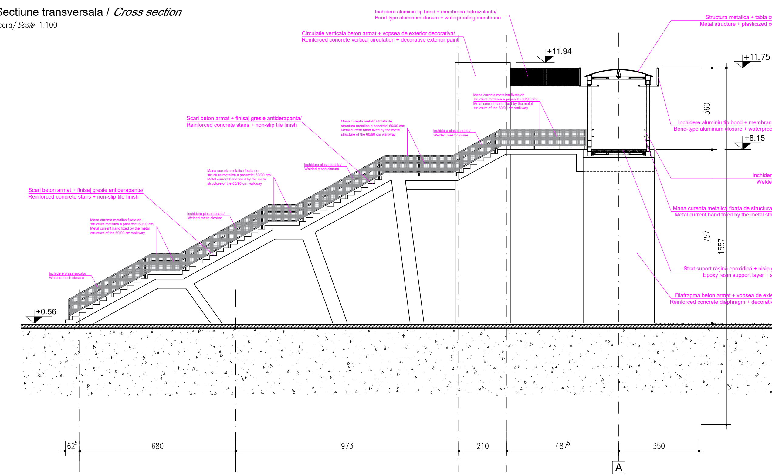
PLAN PASARELA PIETONALA / PEDESTRIAN WALKWAY PLAN Sursa / Scale 1:100
