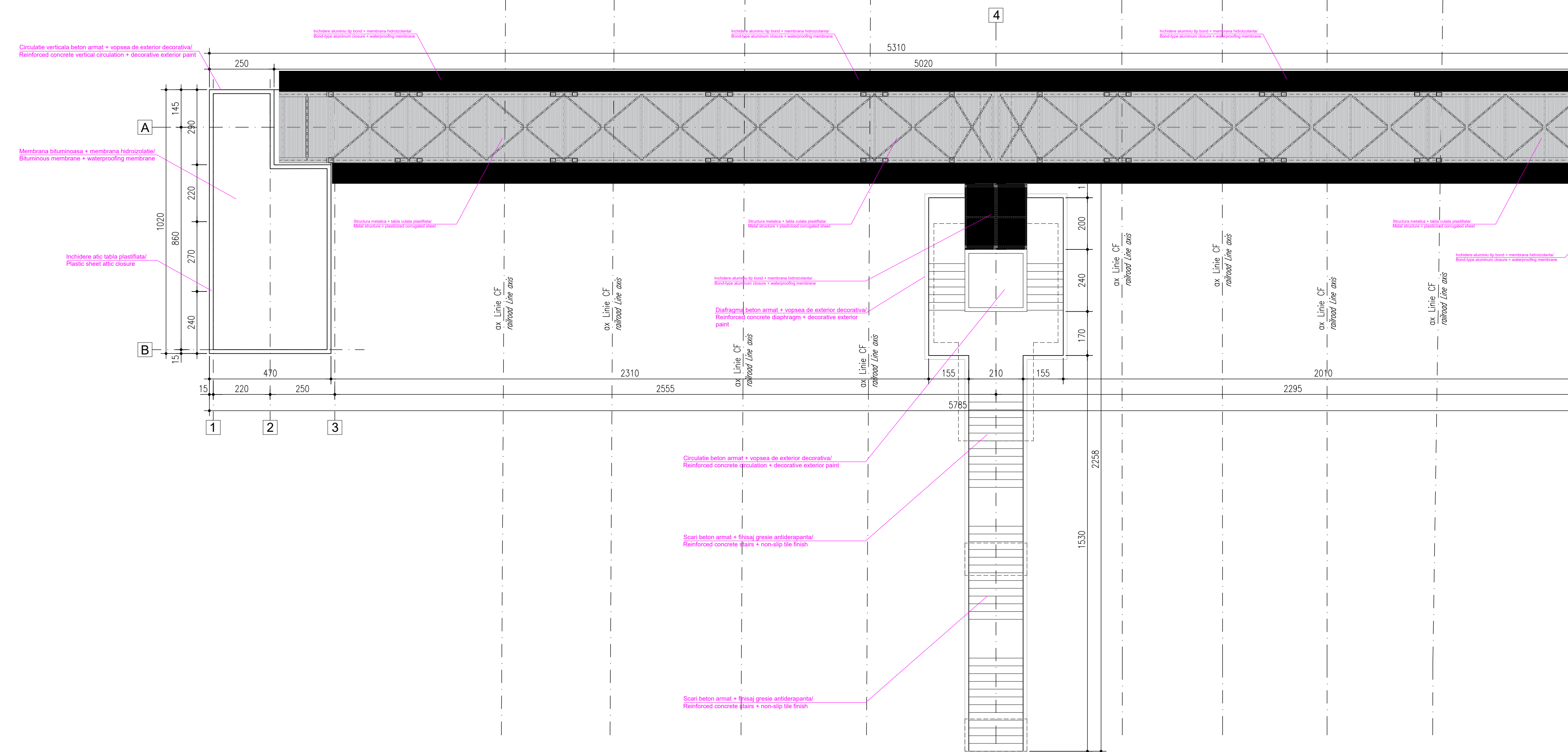
PASARELA PIETONALA / PEDESTRIAN WALKWAY între axe / between axle Sora / Scale 1:100
