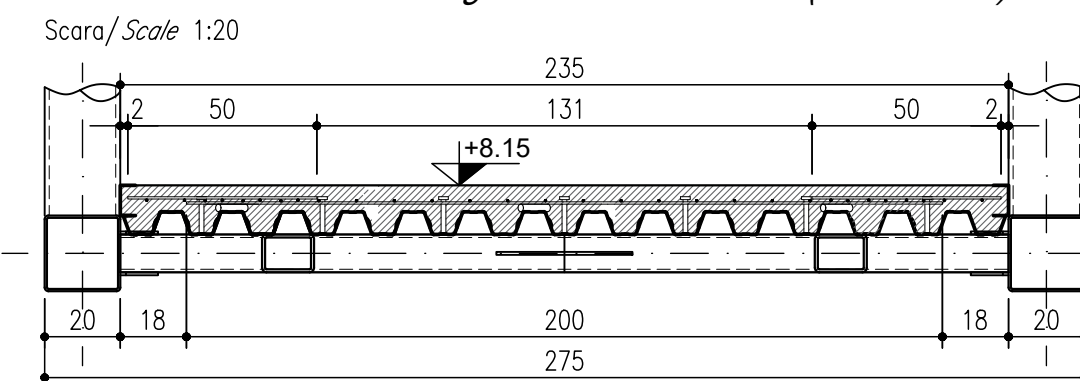
Armare suprabetonare tabla cutata (zona curenta) / Overcast reinforcementcorrugated steel blackboard (current area)
