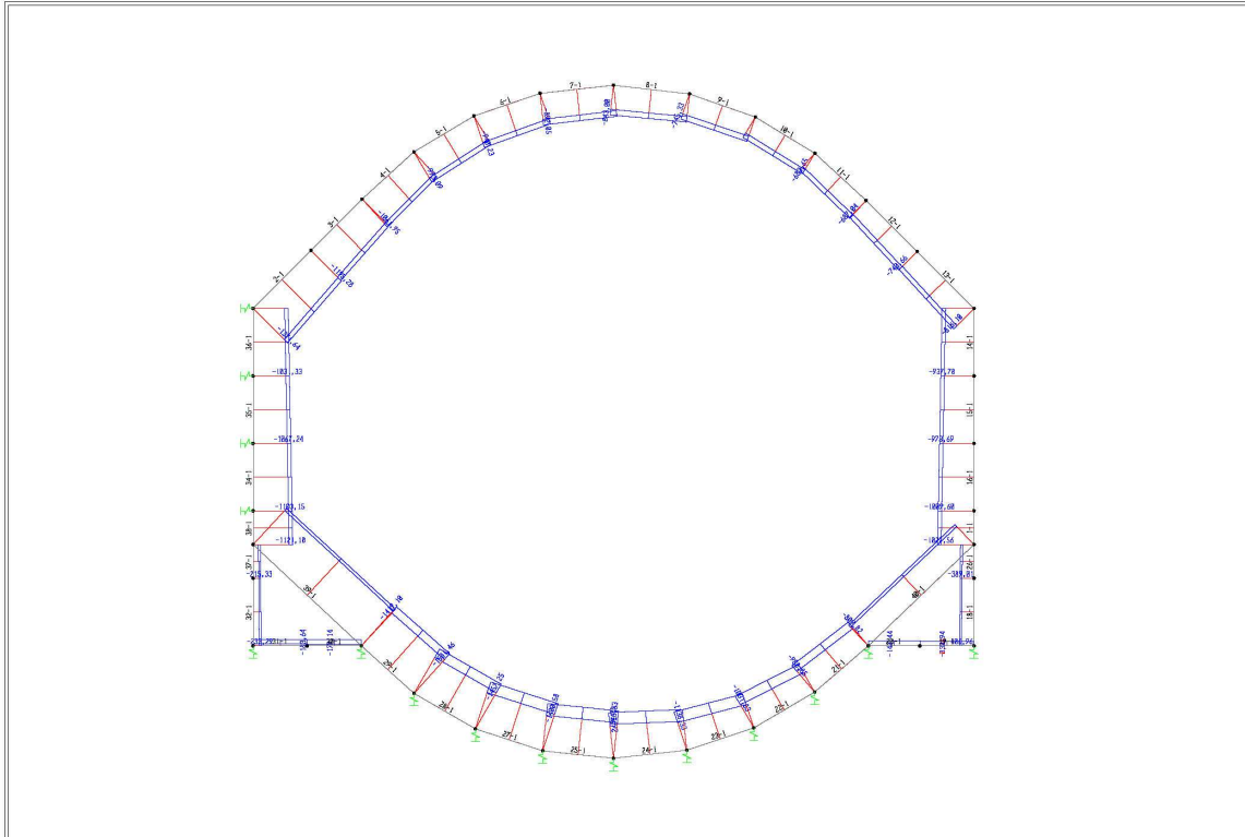
SAP2000 v14.2.2 - File:Ormenis Seismic - Axial Force Diagram (ENVELOPE_ULS) - KN, m, C Units
