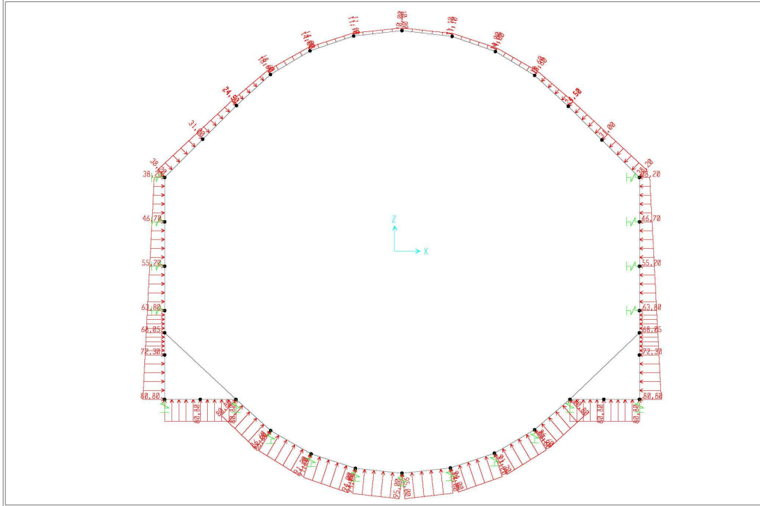
SAP2000 v14.2.2 - File:Ormenis Static - Frame Span Loads (HYDROSTATIC) (As Defined) - KN, m, C Units
