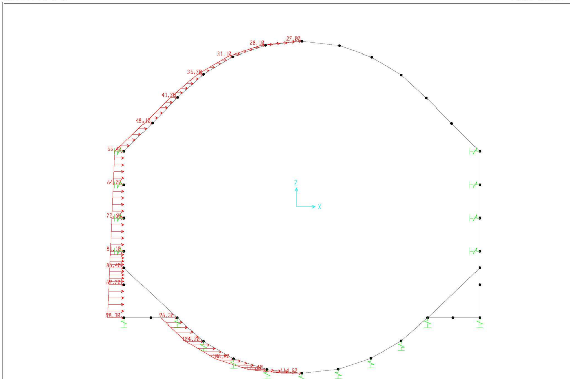
SAP2000 v14.2.2 - File:Ormenis Static - Frame Span Loads (EARTH_PRESSURED_X) (As Defined) - KN, m, C Units
