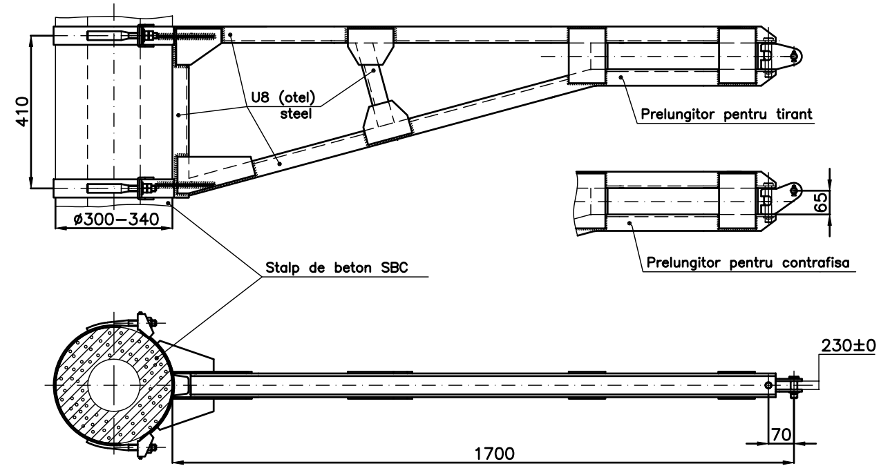
PRELUNGITOR LUNG PE STALP DE BETON SBC LONG STAND-OFF BRACKET FOR CONCRETE POLE SBC
