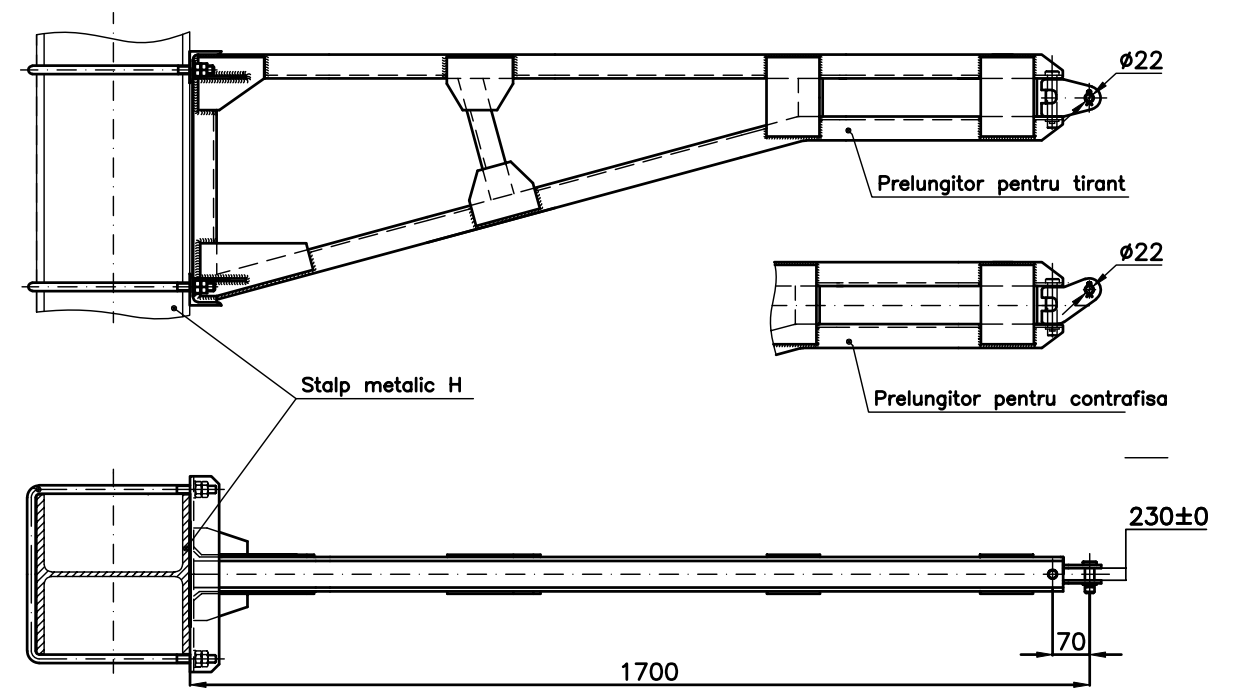
PRELUNGITOR LUNG PE STALP METALIC H LONG STAND-OFF BRACKET FOR METALLICAL POLE TYPE H
