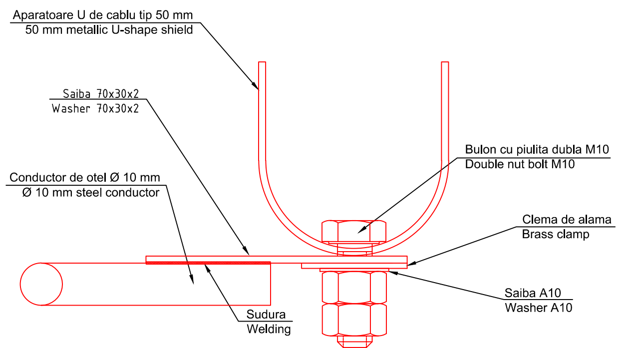
Detaliu de conectare a aparatorii tip U Detail for connection of U shape shield
