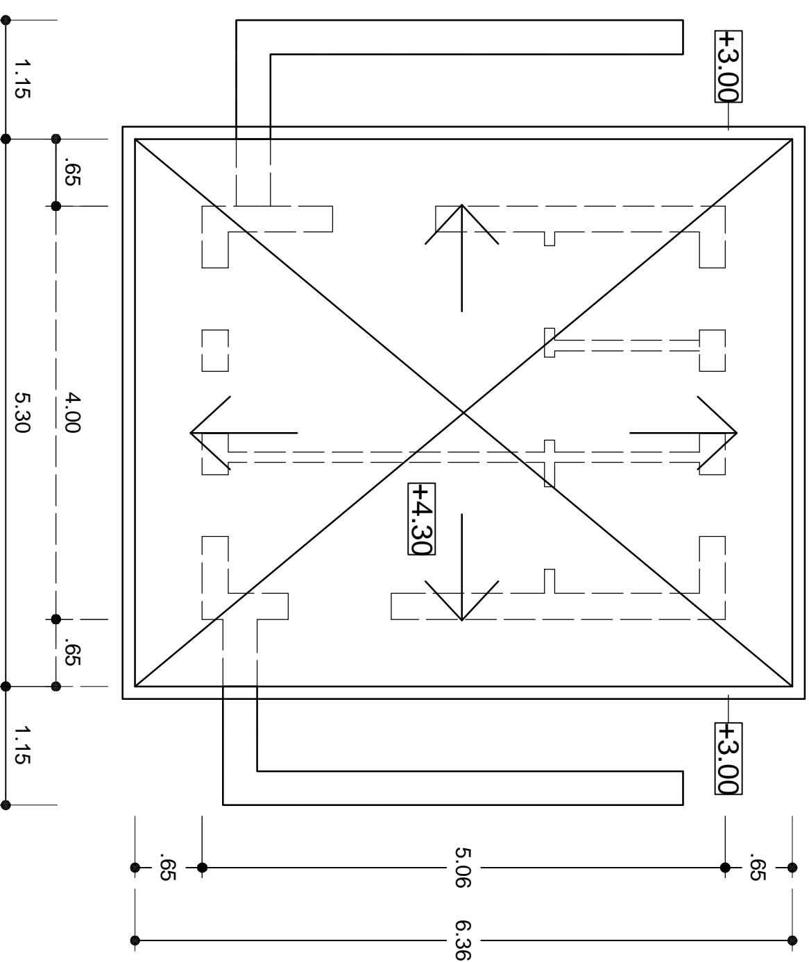
PLAN ACOPERIS - ROOF PLAN SC.1:50
