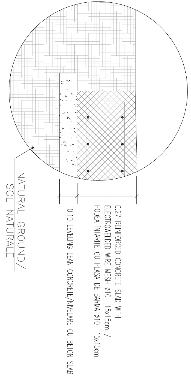
DETAIL/DETALIU "C"
