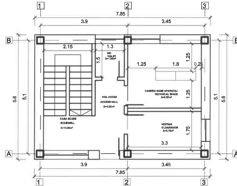
PLAN PARTER GROUND FLOOR PLAN
