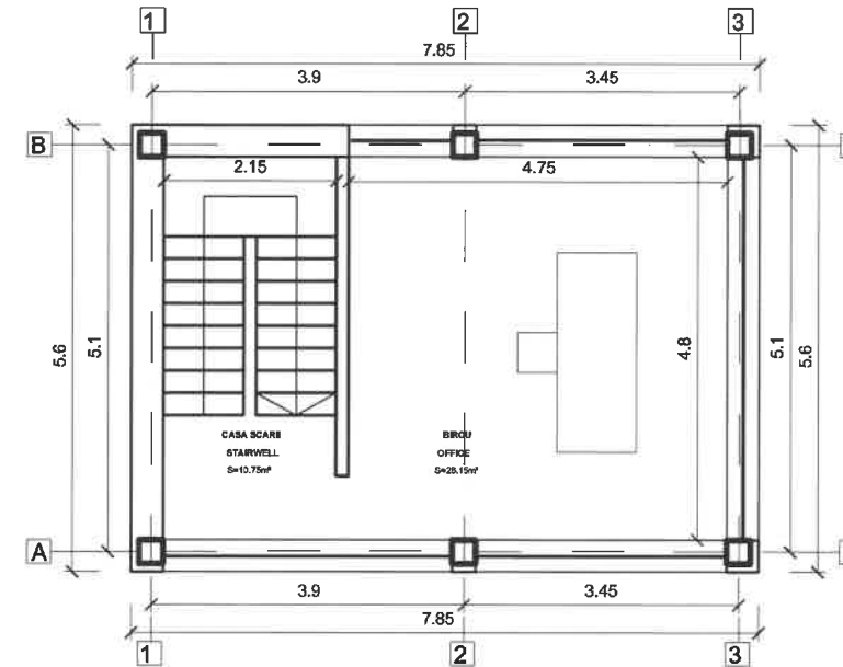
PLAN ETAJ FIRST FLOOR PLAN
