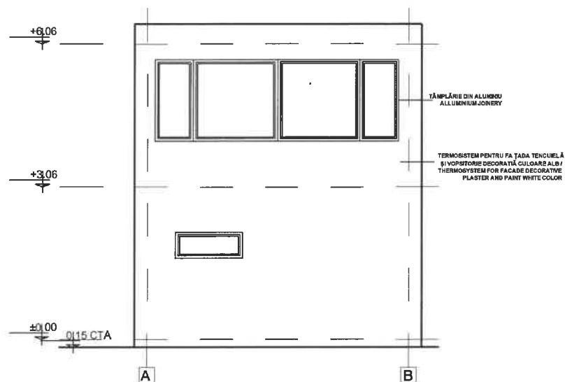
FATADA LATERALA DREAPTA RIGHT SIDE FACADE
