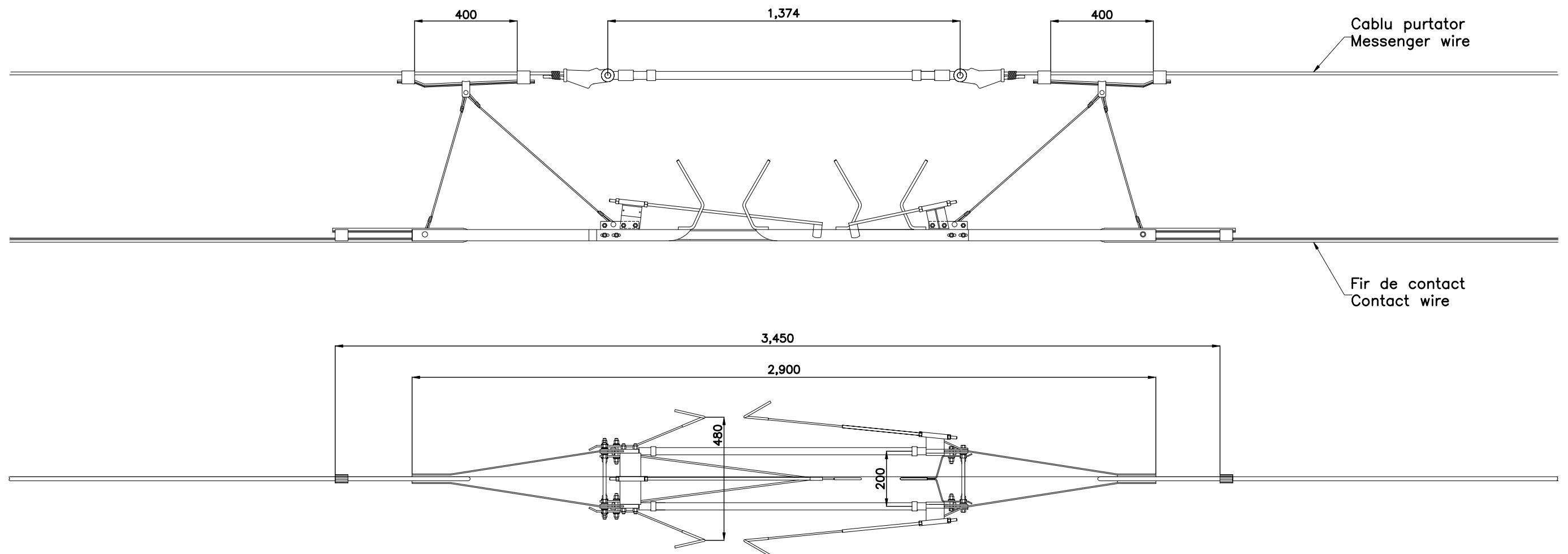
IZOLATOR DE SECTIONARE SECTION INSULATOR
