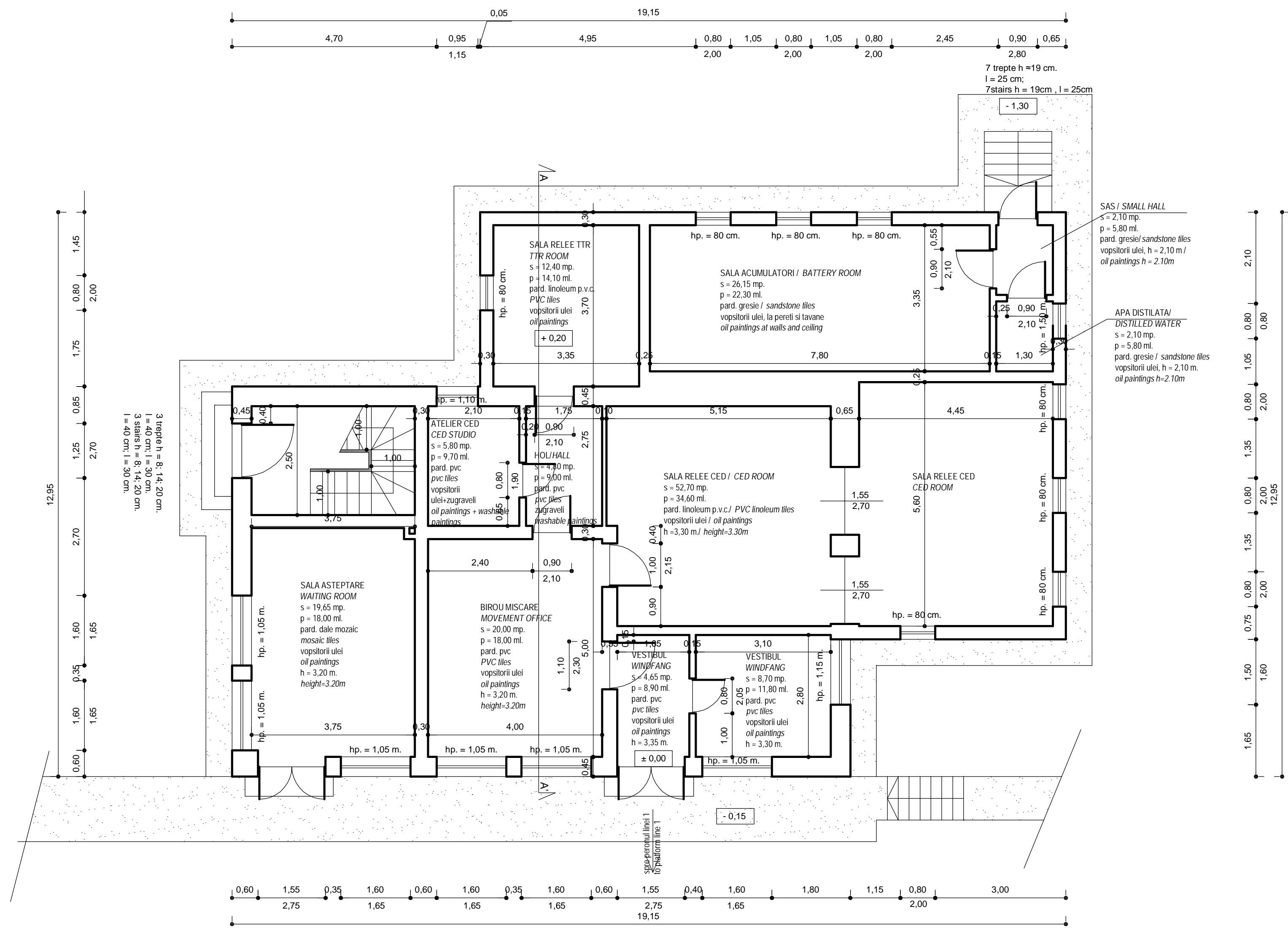
PLAN PARTER SC. 1/50 GROUND FLOOR PLAN SCALE 1/50
