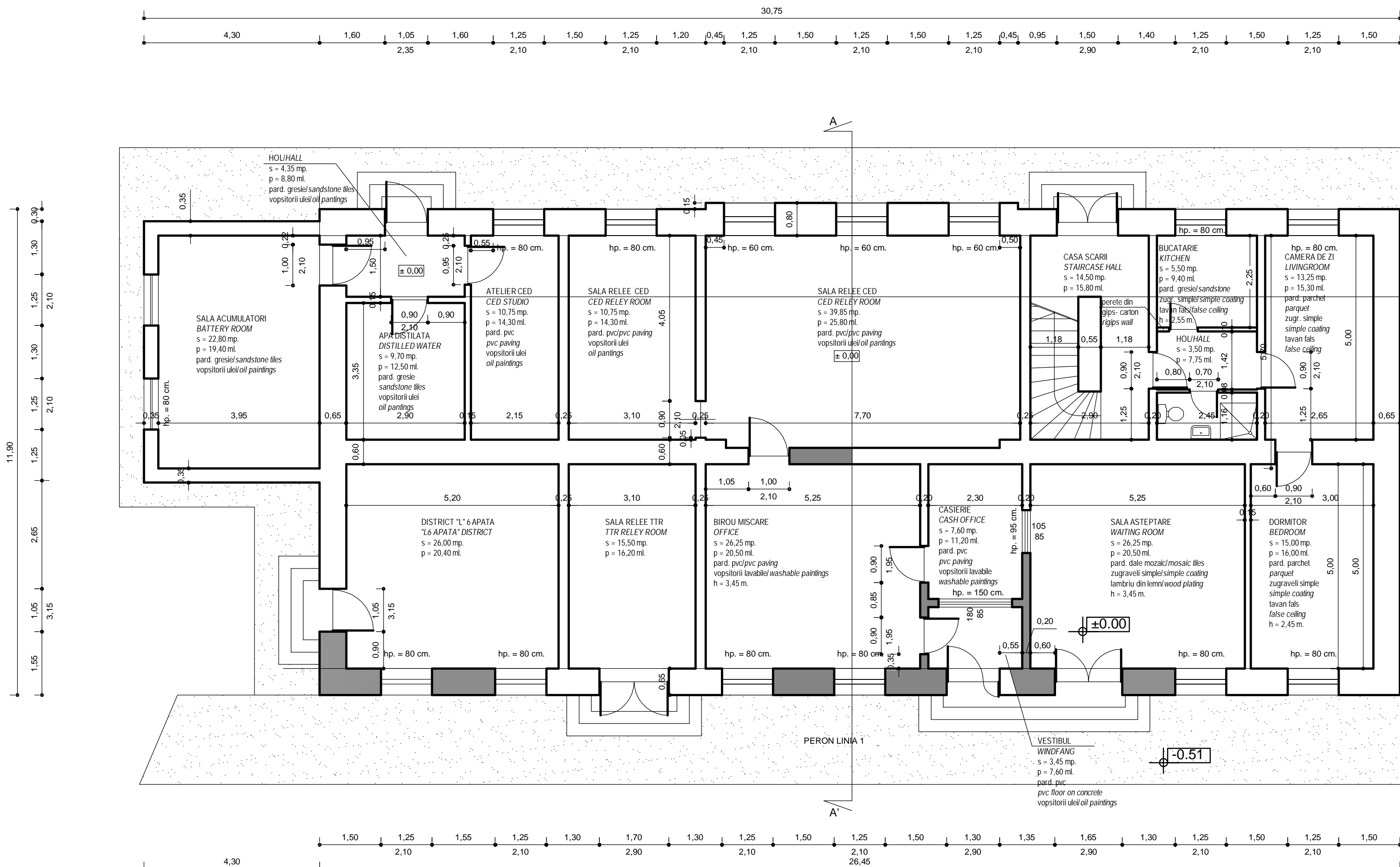
PLAN PARTER SC. 1/50 GROUND FLOOR PLAN SCALE 1/50
