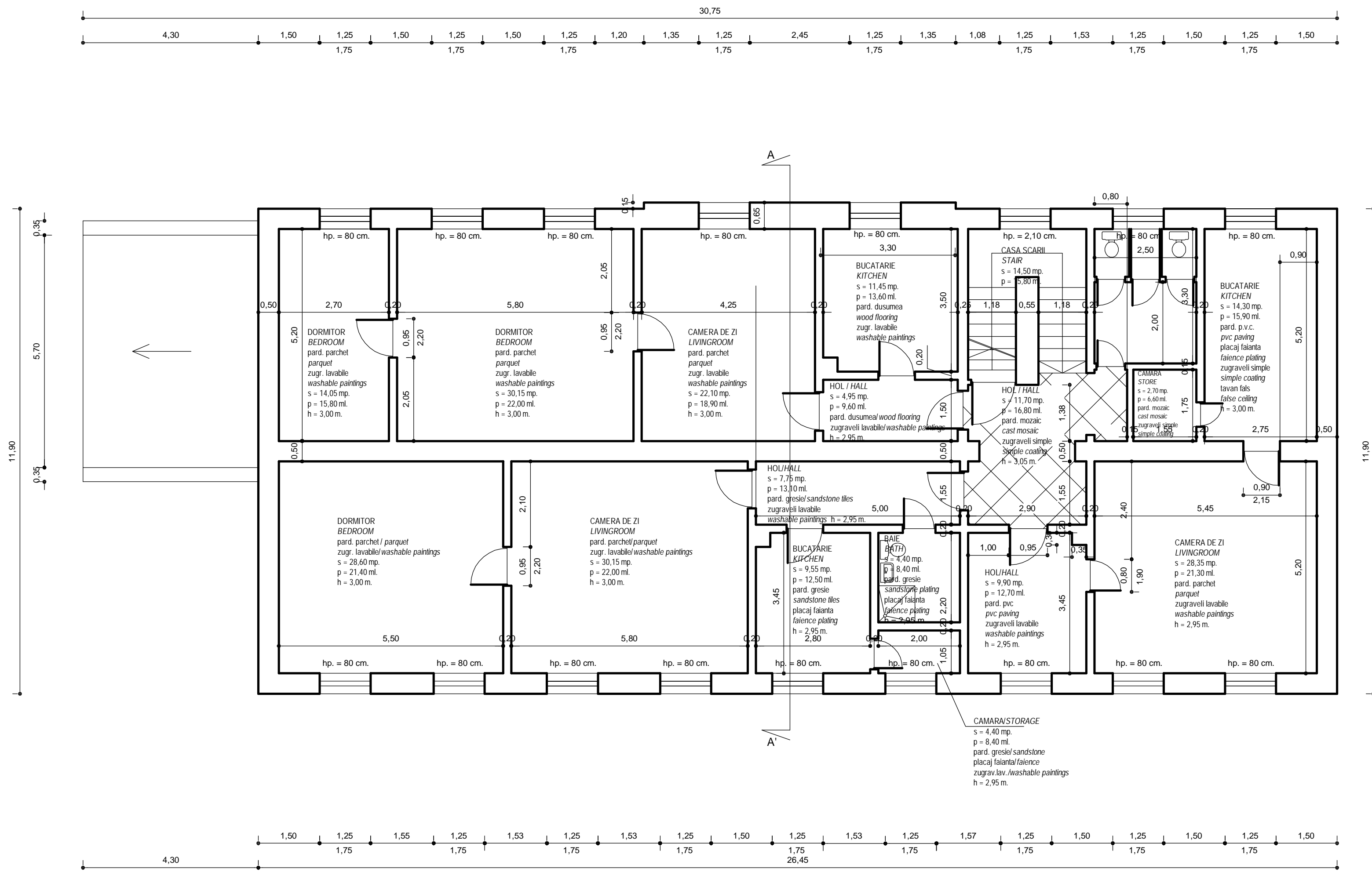
PLAN ETAJ SC. 1/50 FIRST FLOOR PLAN SCALE 1/50
