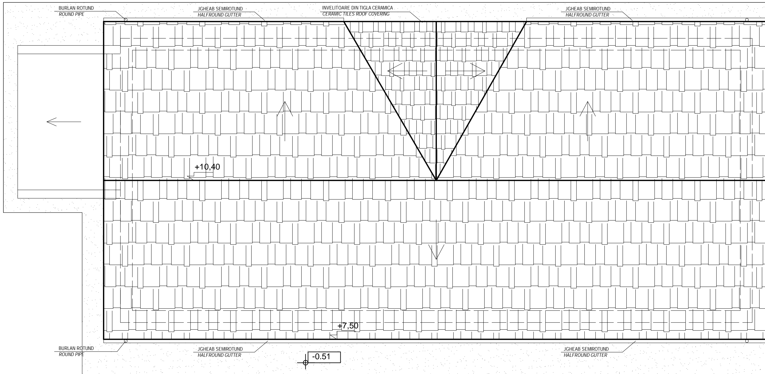
PLAN INVELITOARE SC. 1/50 ROOFTOP PLAN SCALE 1/50
