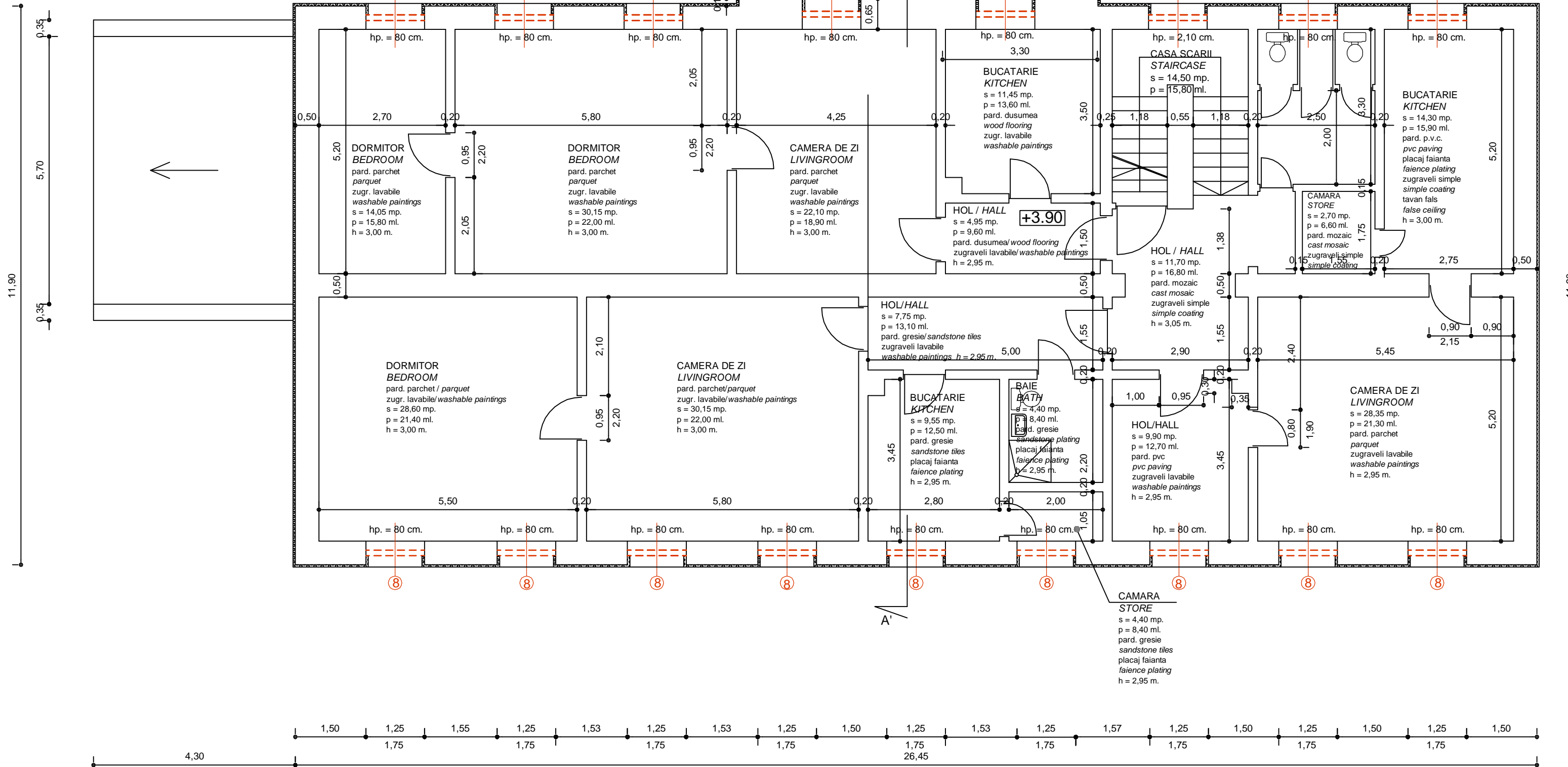
PLAN ETAJ INLOCUIRE TAMPLARIE EXTERIOARA SC. 1/50 FIRST FLOOR PLAN - EXTERIOR WOODWORK REPLACEMENT SCALE 1/50
