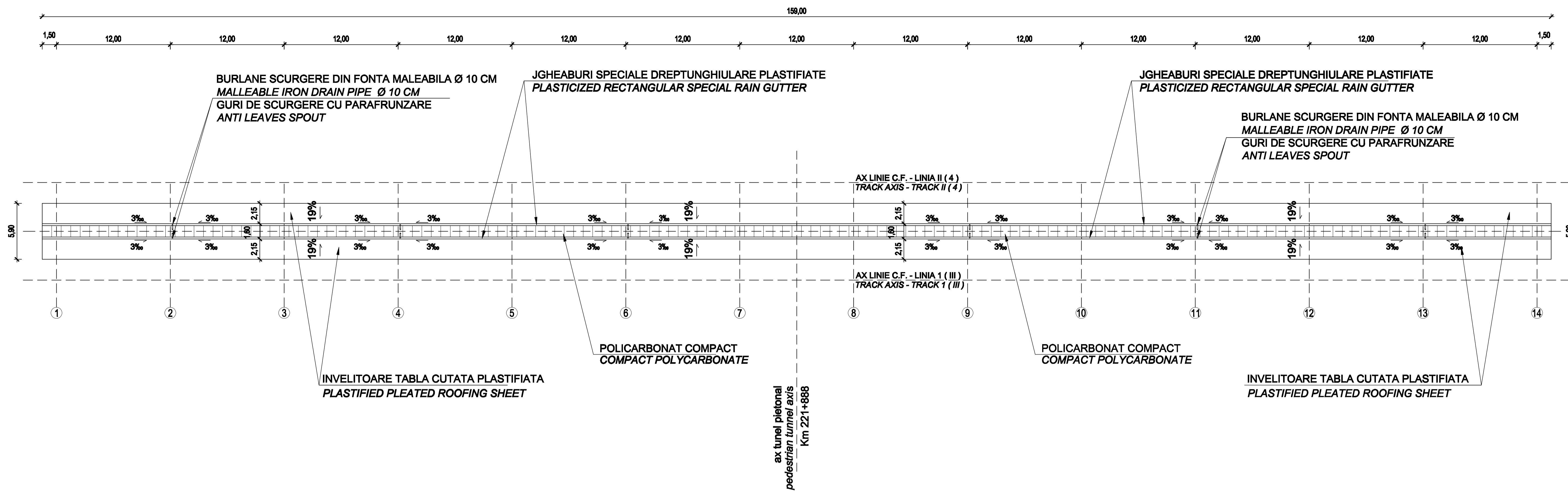
COPERTINE PEROANE INTERMEDIARE scara 1:200 INTERMEDIATE PLATFORMS CANOPY scale 1:200
