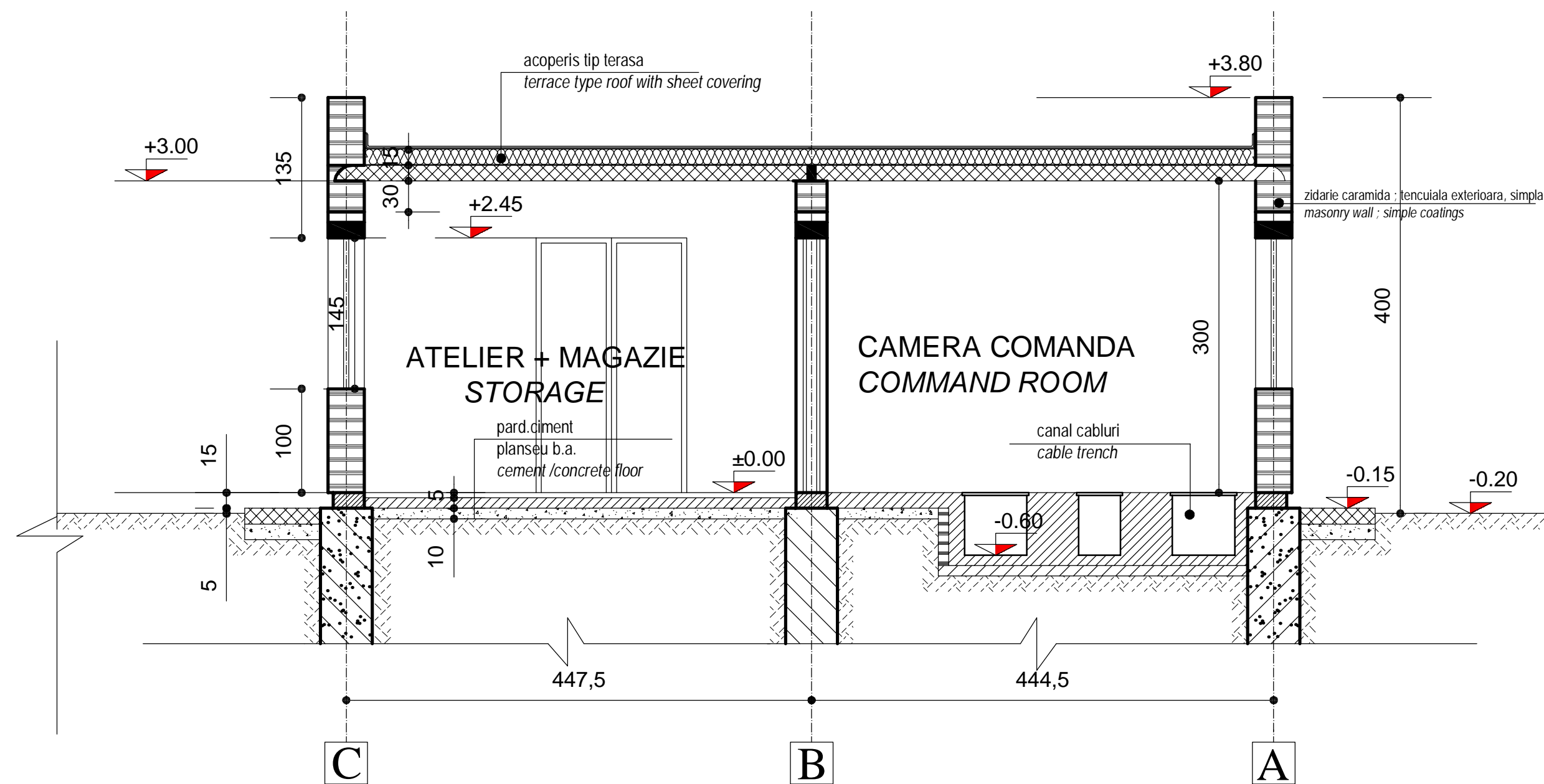
SECTIUNE TRANSVERSALA "A" - "A" Scara 1:50 CROSS SECTION
