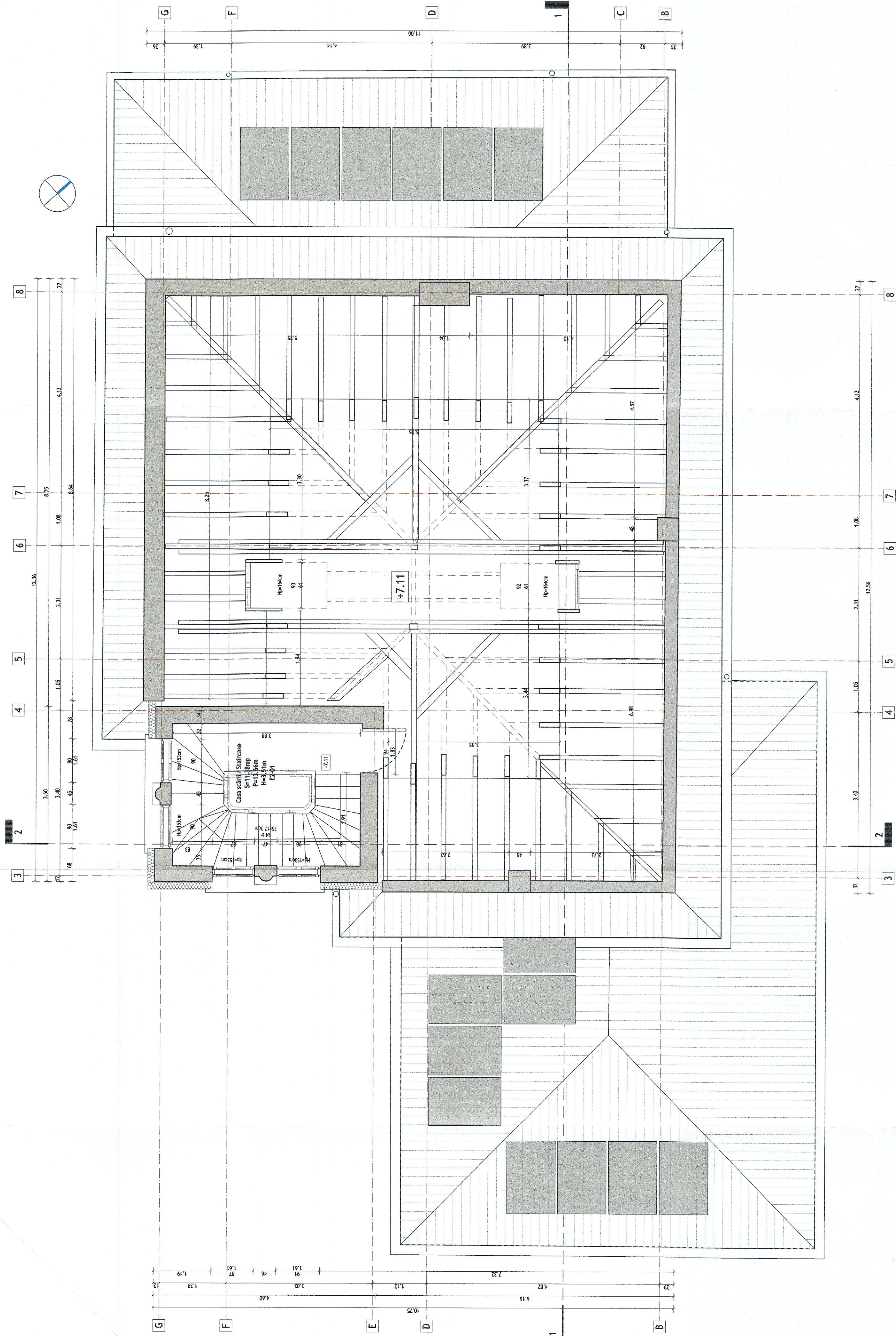
Plan etaj 2 / Second floor plan
