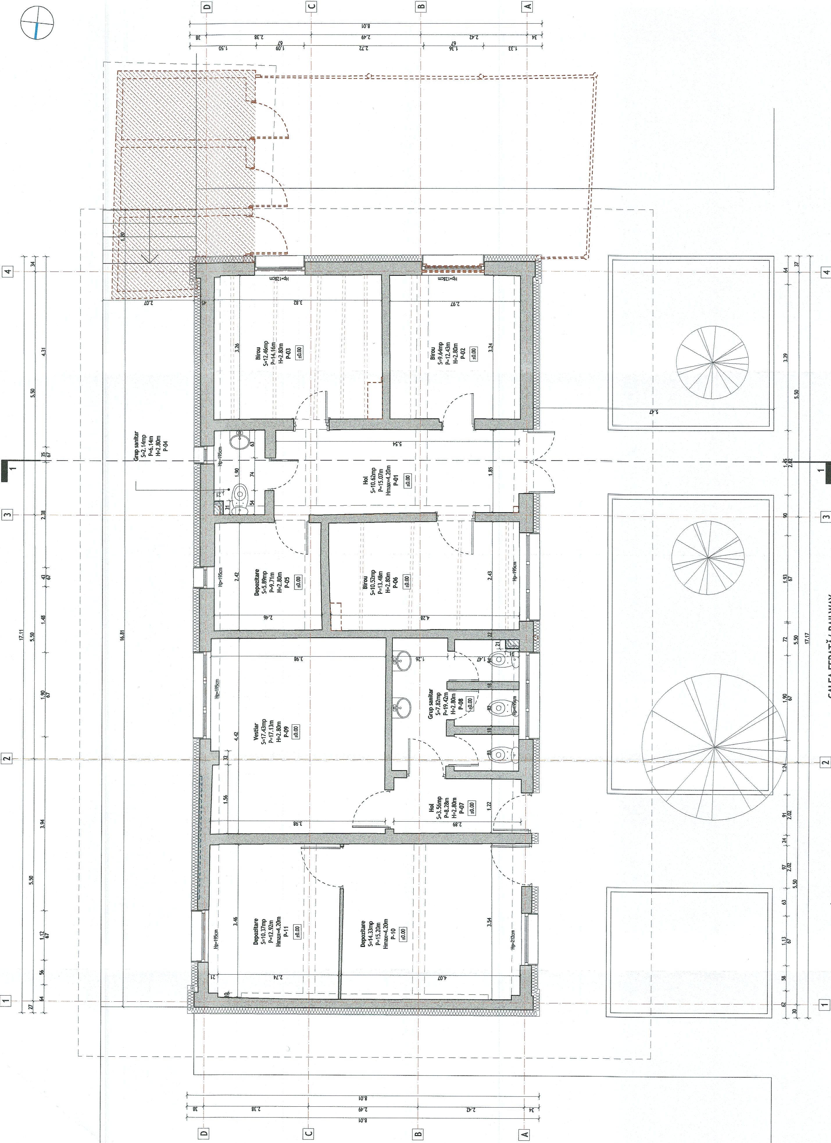
Plan parter/ Ground floor plan
