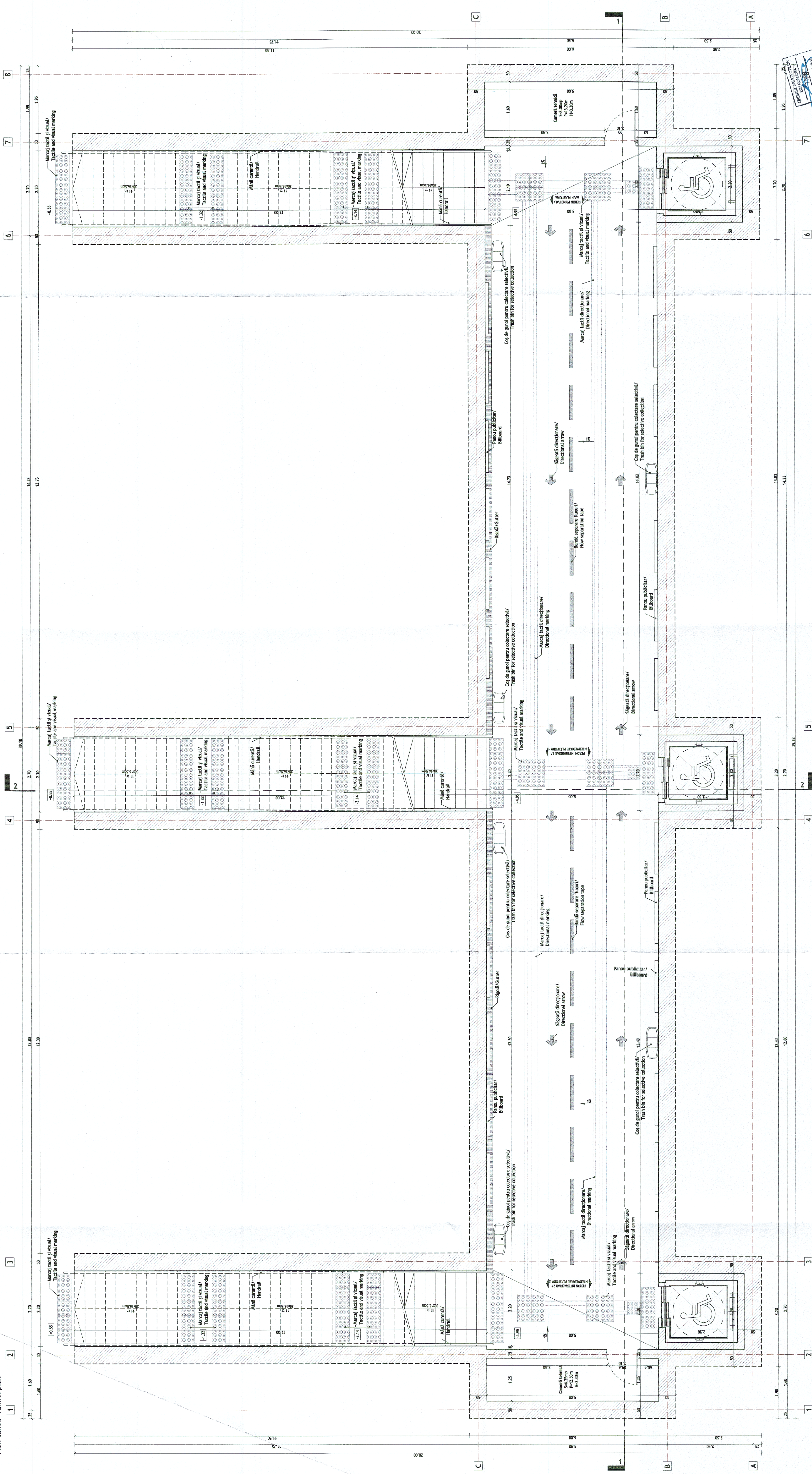
Plan tunnel/ Tunnel plan
