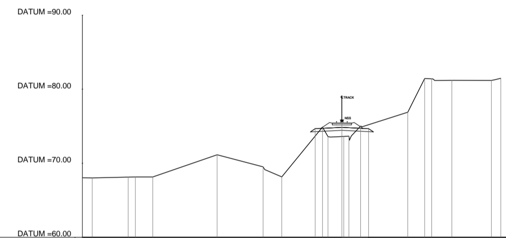
KM.383+620.00 SEC. 502
