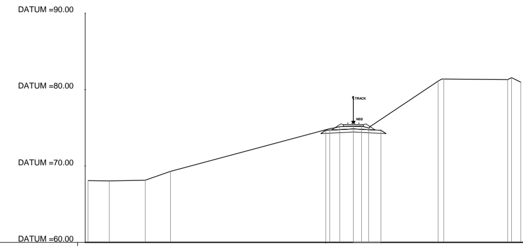
KM.383+600.00 SEC. 501
