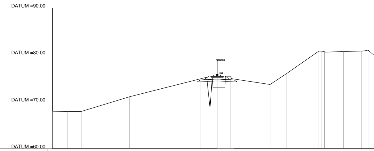
KM.383+755.00 SEC. 504
