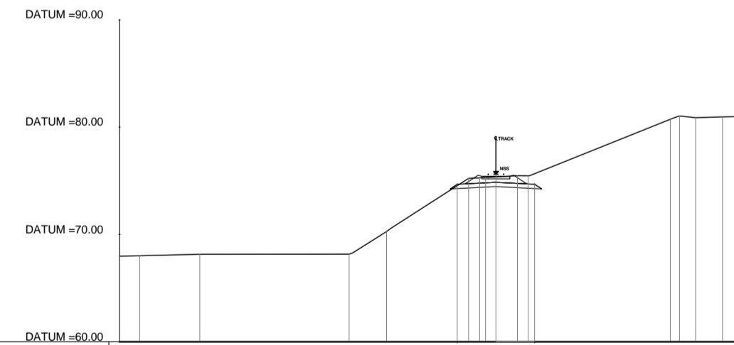
KM.383+689.00 SEC. 503
