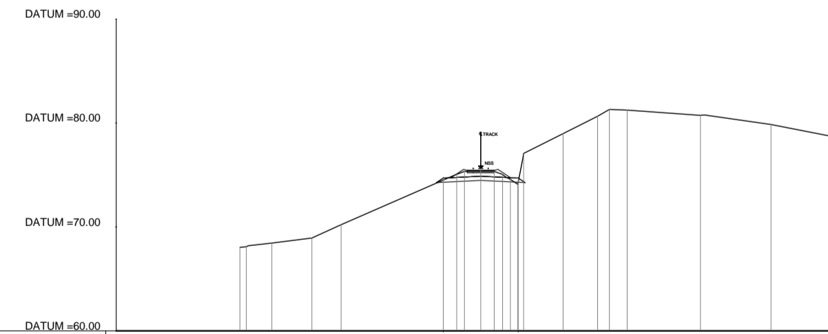
KM.384+000.00 SEC. 506
